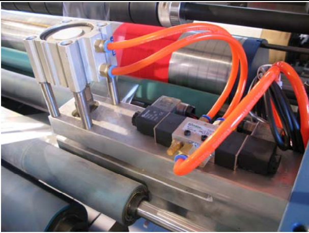
Film Punching unit(2-side window box)
