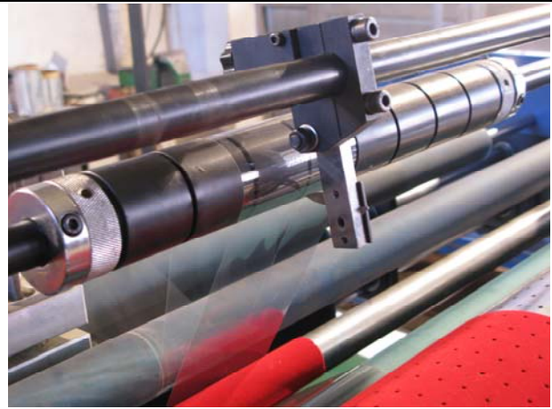
Film Cutting(tissue box)
